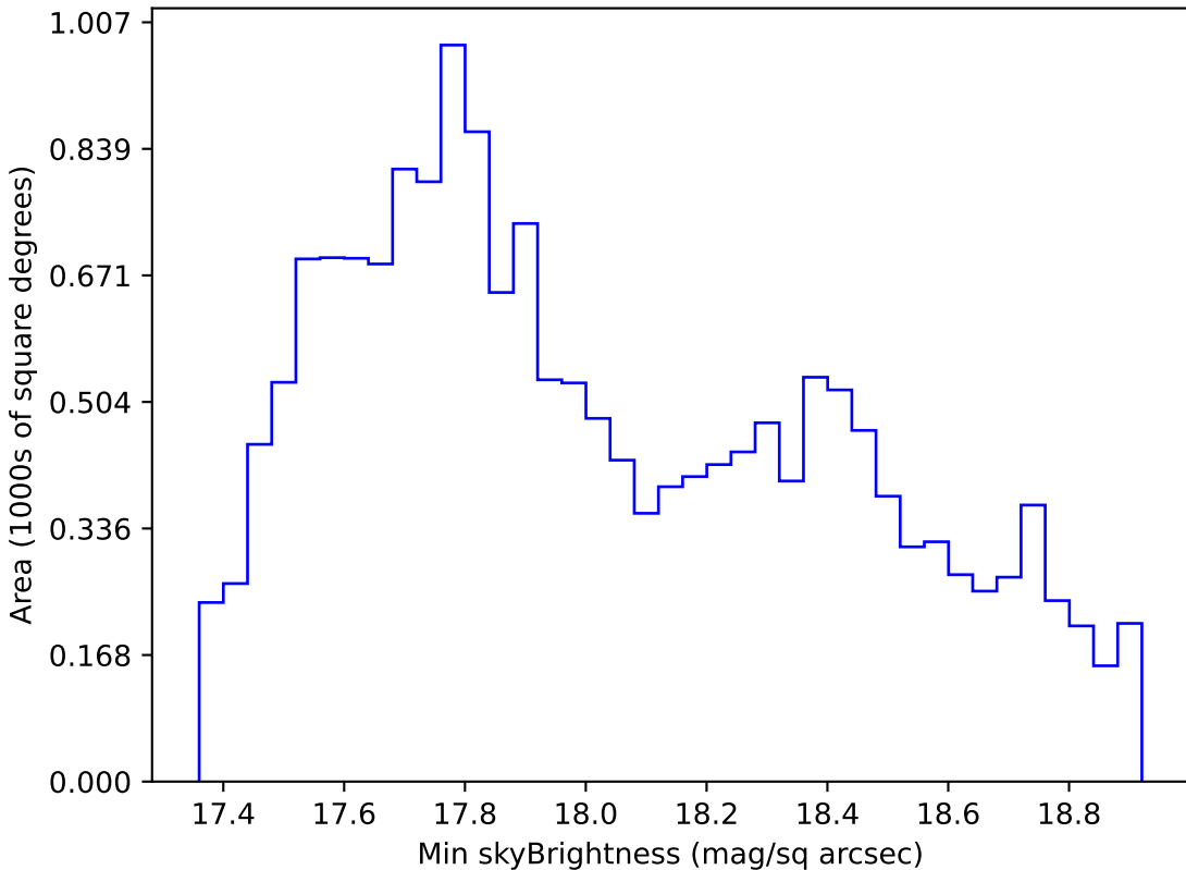
too_10_1v3.4_10yrs WFD i band: Min skyBrightness
