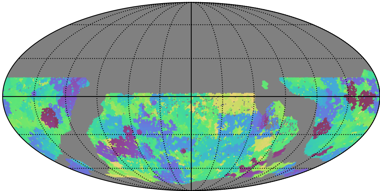
too_10_1v3.4_10yrs WFD g band: Min skyBrightness
