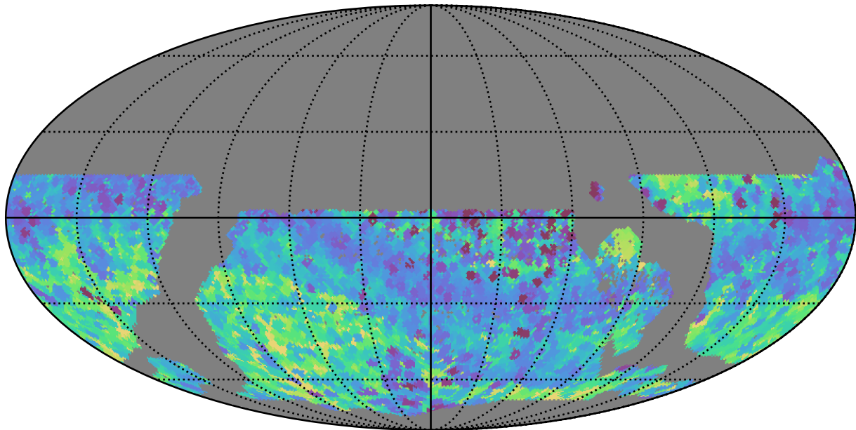
too_10_1v3.4_10yrs WFD all bands: Min skyBrightness
