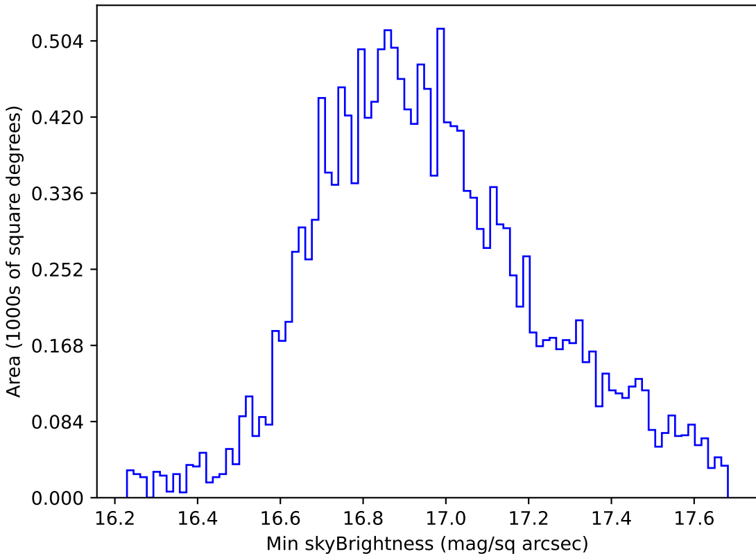
too_10_1v3.4_10yrs WFD all bands: Min skyBrightness
