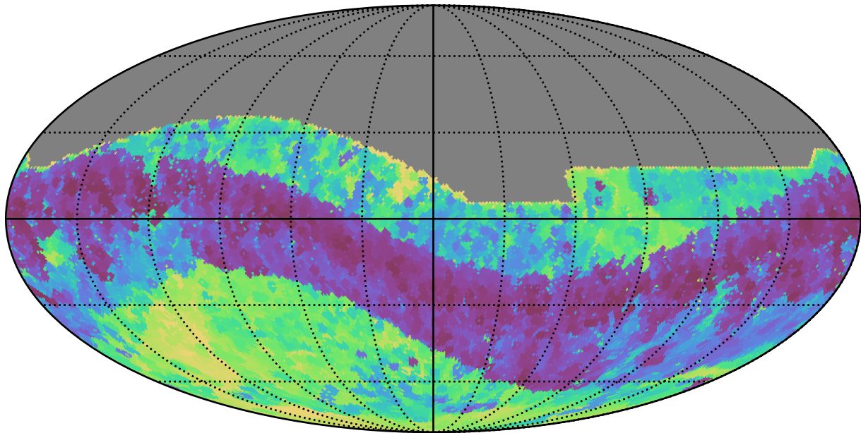
too_10_1v3.4_10yrs All sky z band: Min skyBrightness
