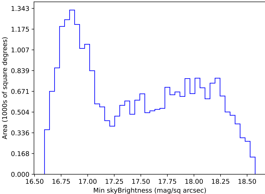
too_10_1v3.4_10yrs All sky z band: Min skyBrightness
