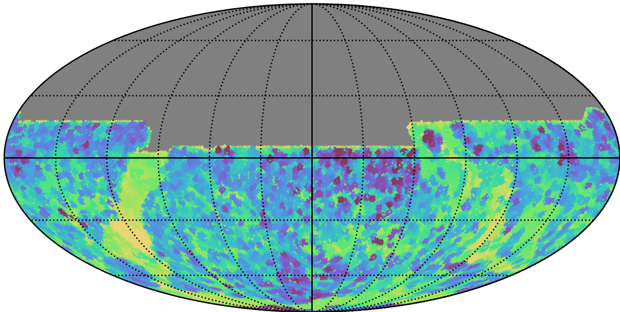
too_10_1v3.4_10yrs All sky y band: Min skyBrightness
