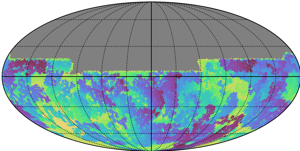
too_10_1v3.4_10yrs All sky u band: Min skyBrightness
