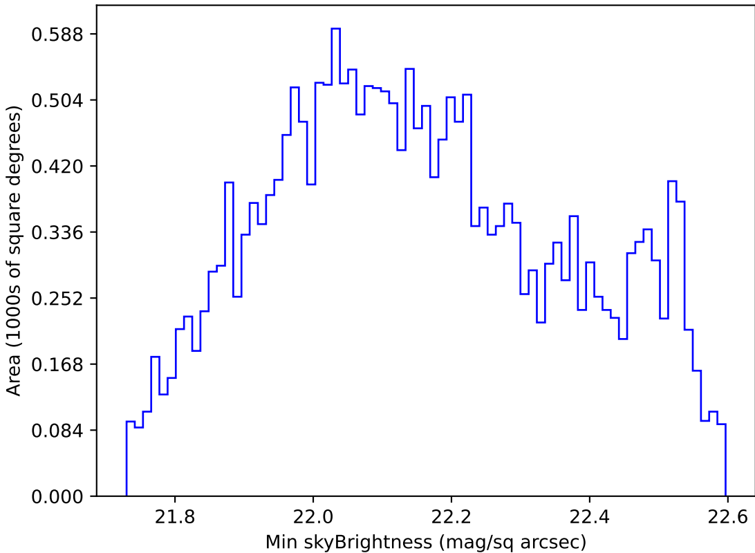
too_10_1v3.4_10yrs All sky u band: Min skyBrightness
