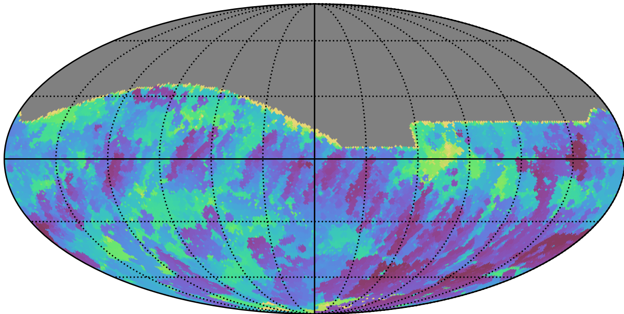
too_10_1v3.4_10yrs All sky r band: Min skyBrightness
