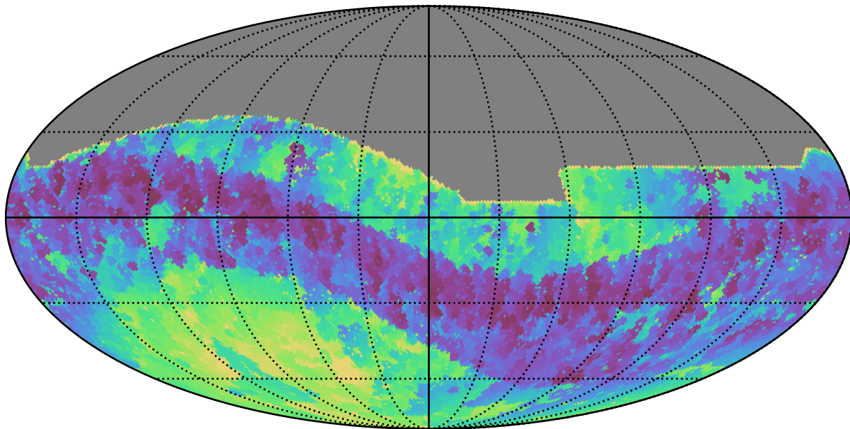
too_10_1v3.4_10yrs All sky i band: Min skyBrightness
