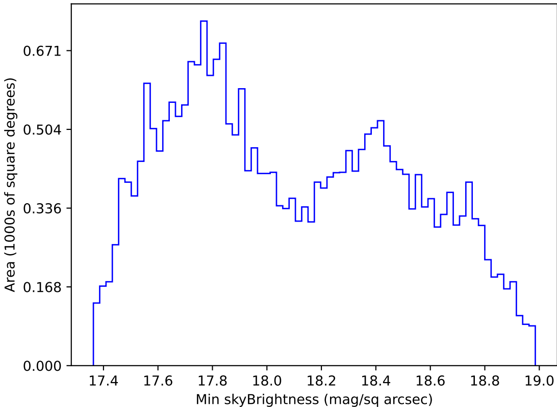
too_10_1v3.4_10yrs All sky i band: Min skyBrightness
