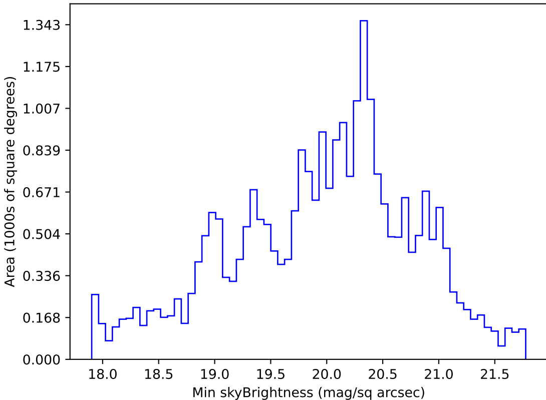
too_10_1v3.4_10yrs All sky g band: Min skyBrightness
