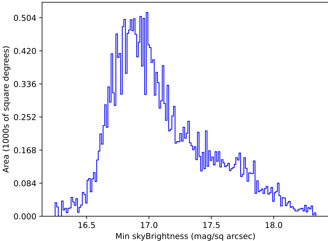
too_10_1v3.4_10yrs All sky all bands: Min skyBrightness
