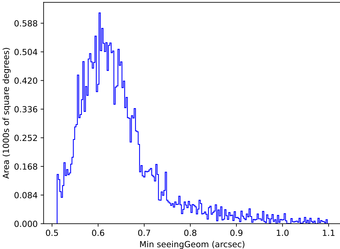
too_10_1v3.4_10yrs Yr 1 z band: Min seeingGeom
