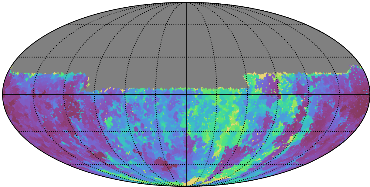
too_10_1v3.4_10yrs Yr 1 u band: Min seeingGeom
