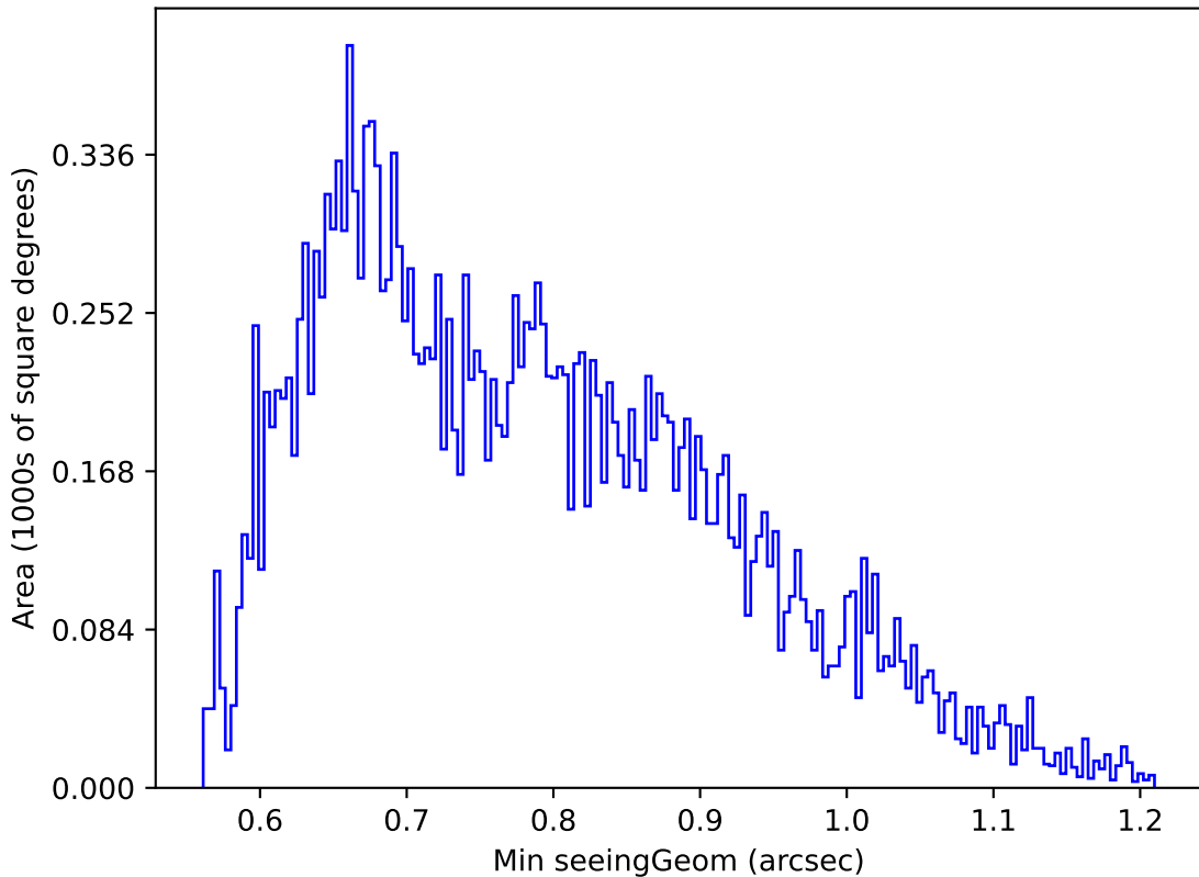
too_10_1v3.4_10yrs Yr 1 u band: Min seeingGeom
