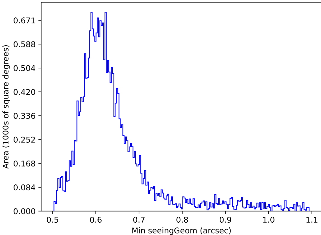
too_10_1v3.4_10yrs Yr 1 r band: Min seeingGeom
