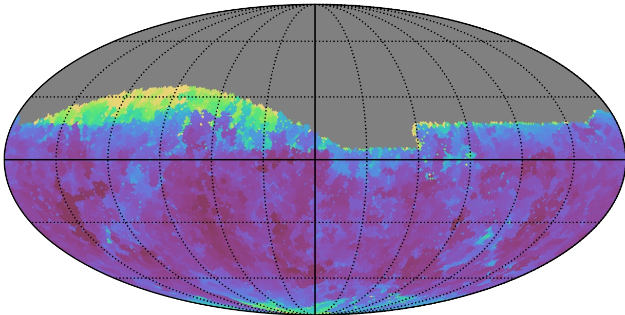
too_10_1v3.4_10yrs Yr 1 i band: Min seeingGeom
