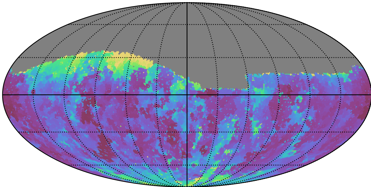
too_10_1v3.4_10yrs Yr 1 g band: Min seeingGeom
