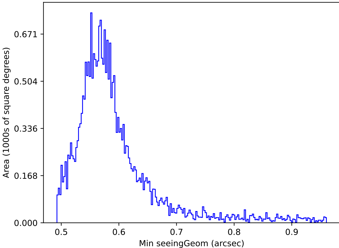
too_10_1v3.4_10yrs Yr 1 all bands: Min seeingGeom
