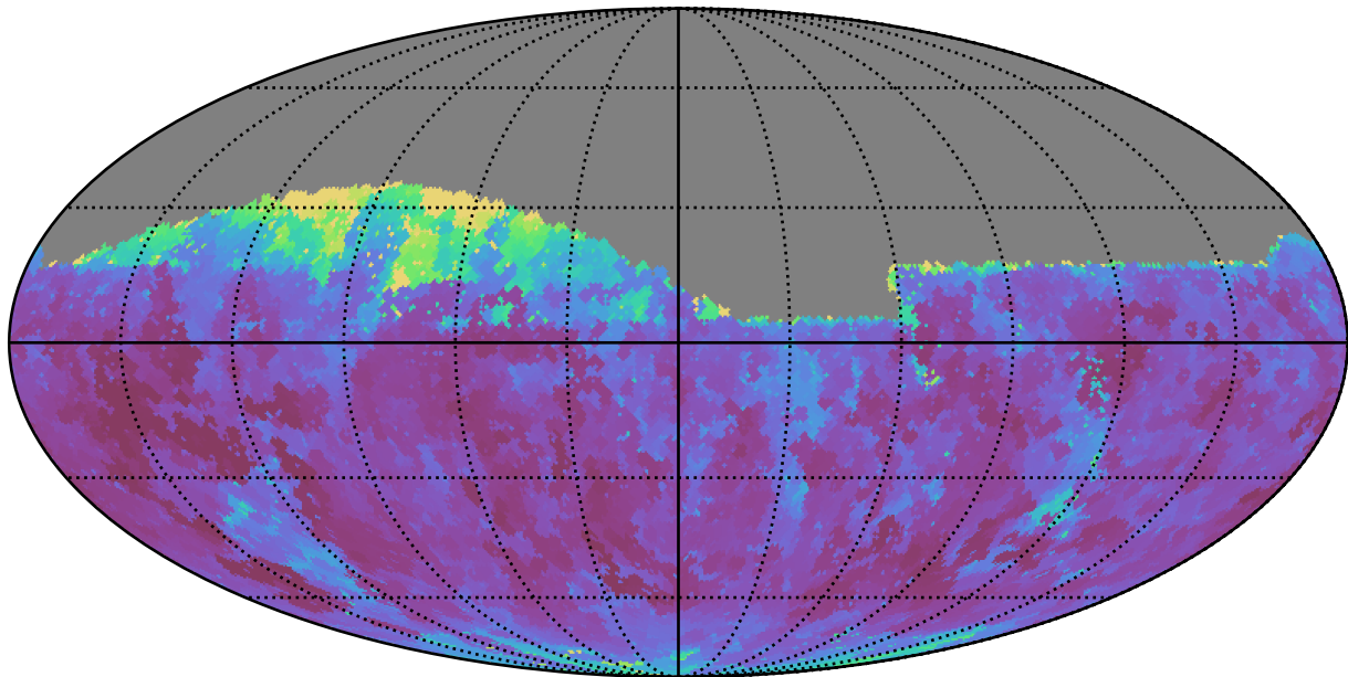
too_10_1v3.4_10yrs Yr 1 z band: Min seeingEff
