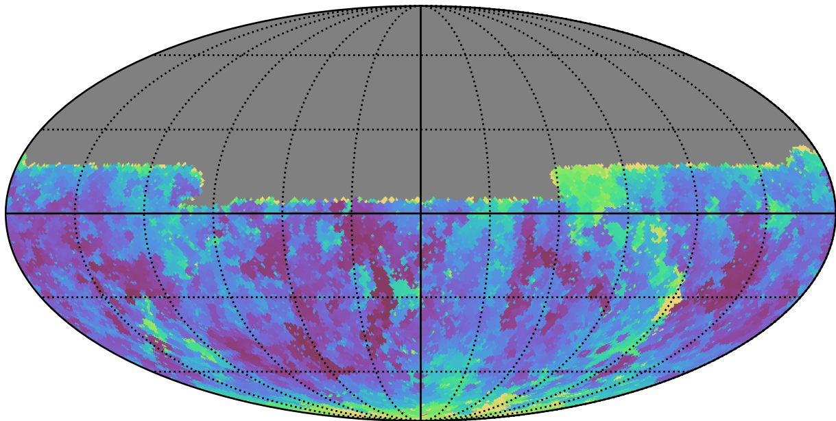
too_10_1v3.4_10yrs Yr 1 y band: Min seeingEff
