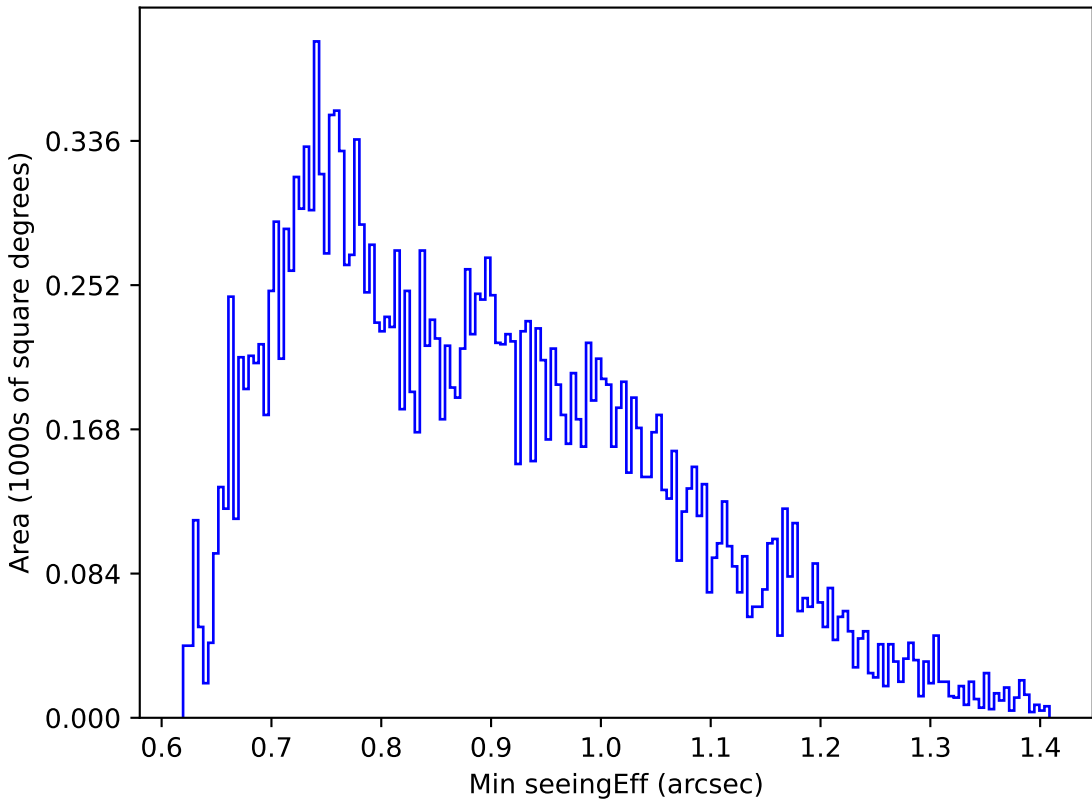
too_10_1v3.4_10yrs Yr 1 u band: Min seeingEff
