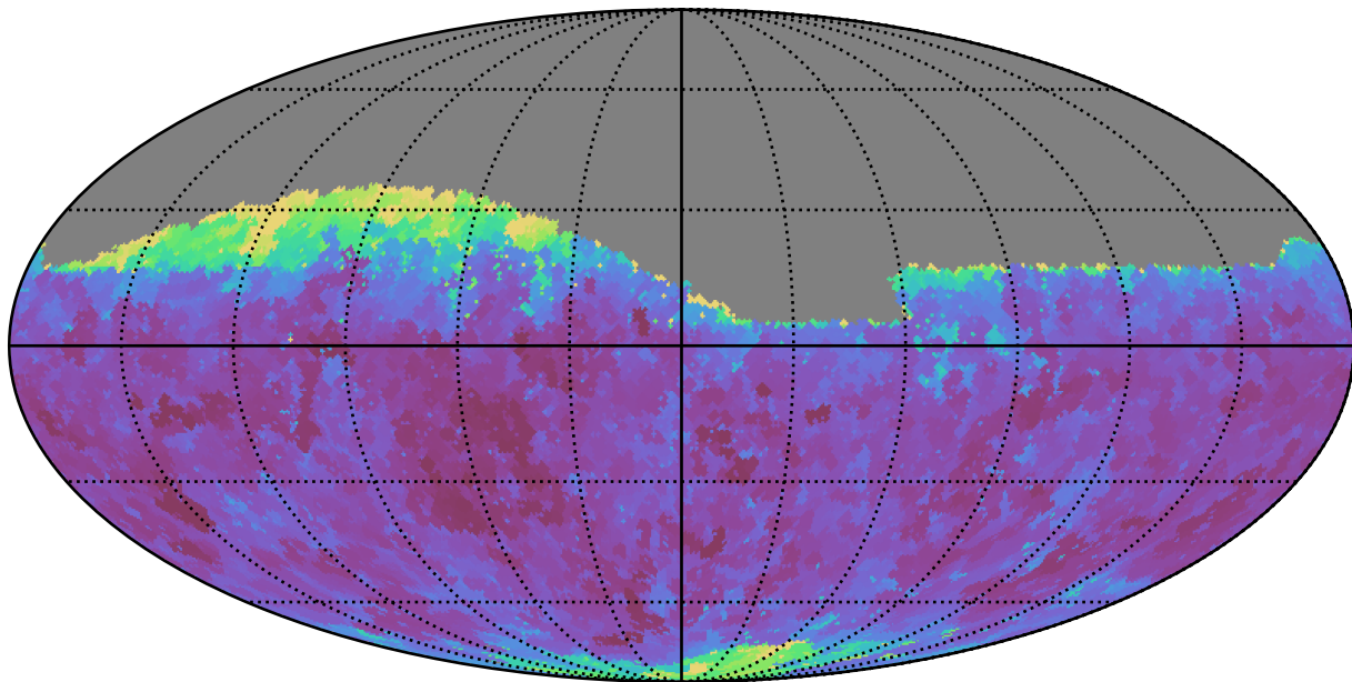
too_10_1v3.4_10yrs Yr 1 r band: Min seeingEff
