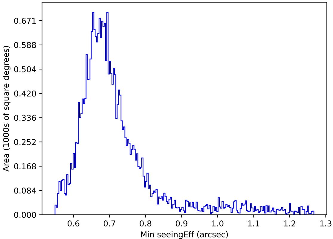
too_10_1v3.4_10yrs Yr 1 r band: Min seeingEff
