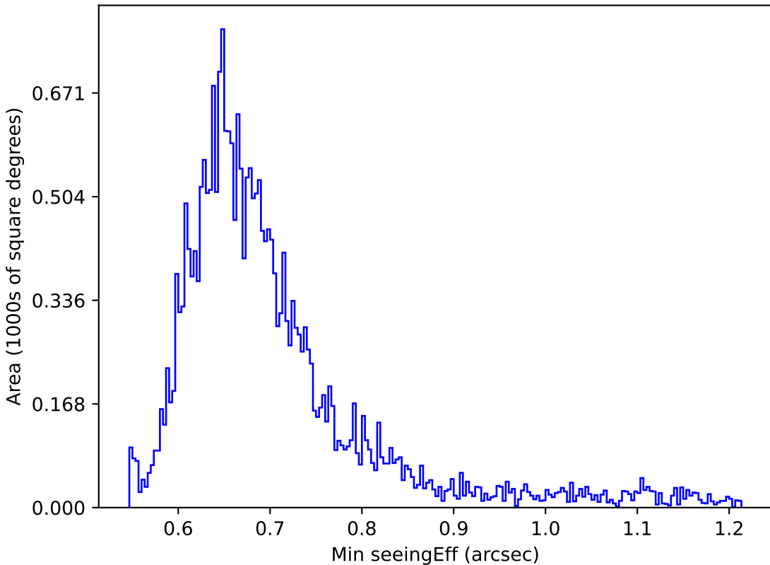
too_10_1v3.4_10yrs Yr 1 i band: Min seeingEff
