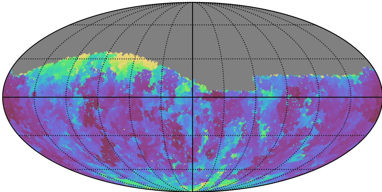
too_10_1v3.4_10yrs Yr 1 g band: Min seeingEff
