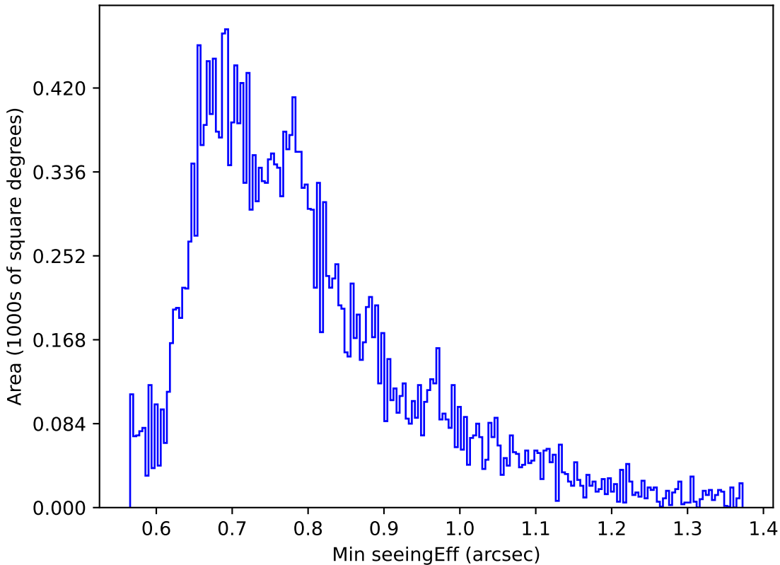
too_10_1v3.4_10yrs Yr 1 g band: Min seeingEff
