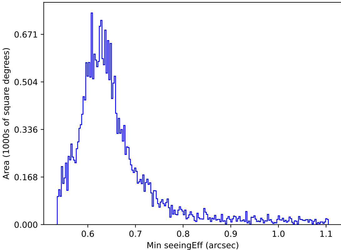
too_10_1v3.4_10yrs Yr 1 all bands: Min seeingEff
