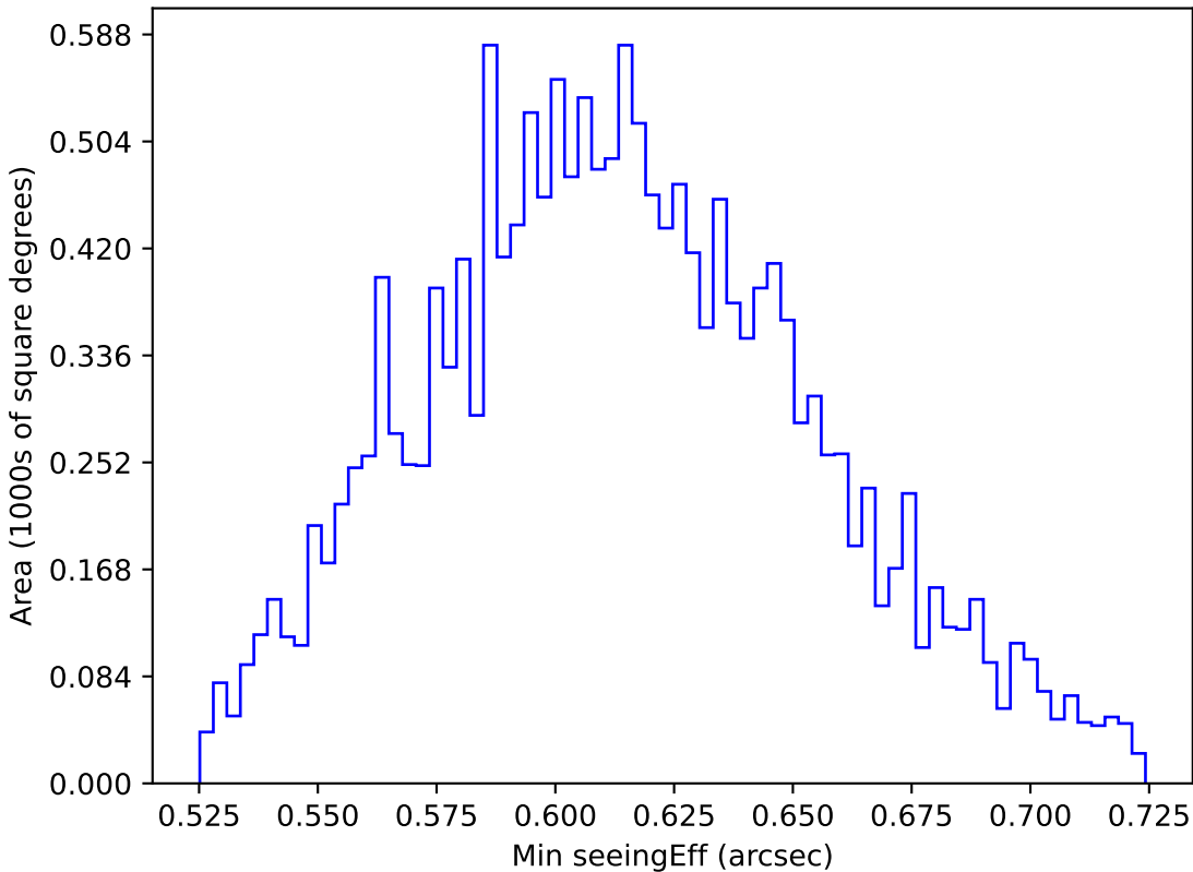
too_10_1v3.4_10yrs WFD z band: Min seeingEff
