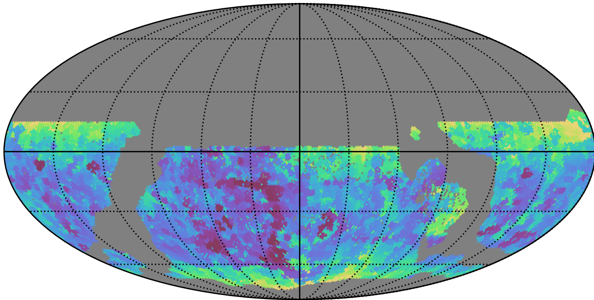
too_10_1v3.4_10yrs WFD y band: Min seeingEff
