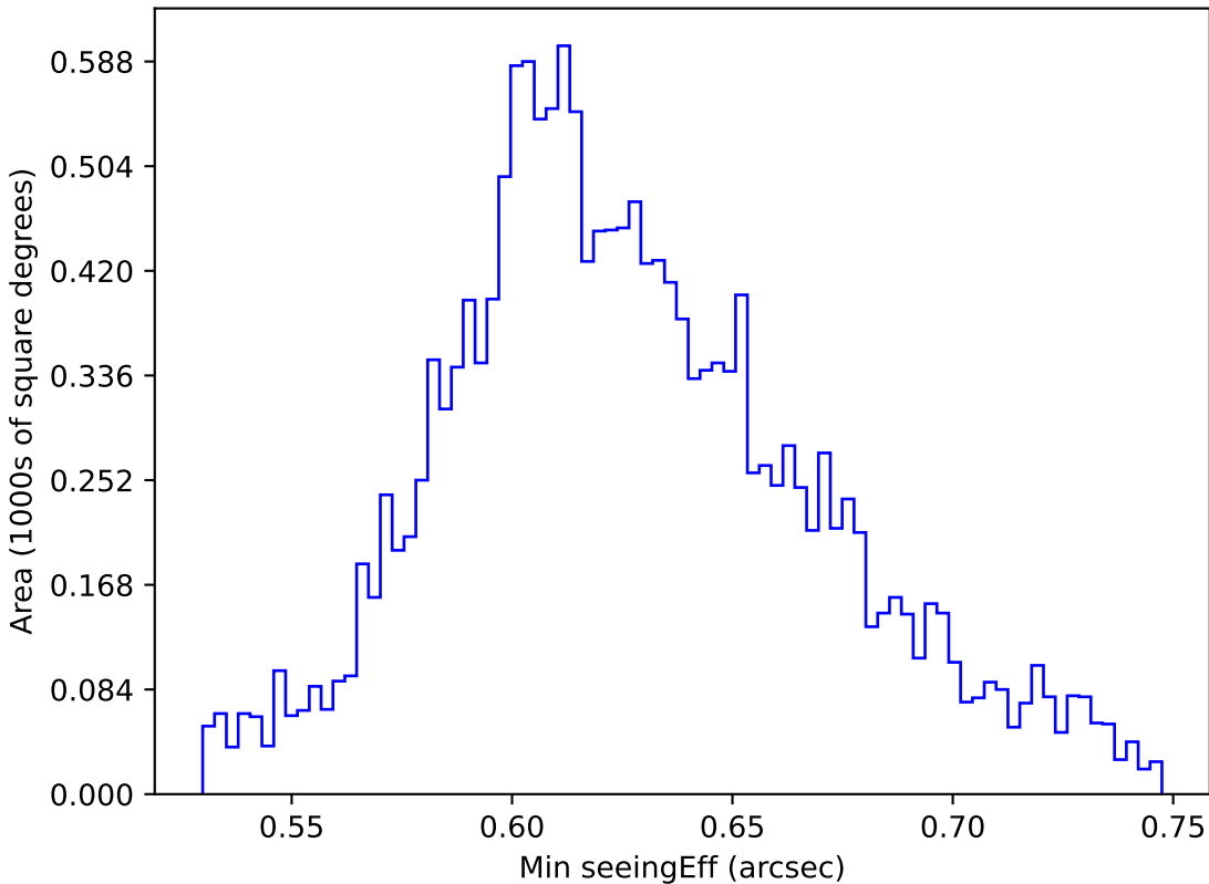
too_10_1v3.4_10yrs WFD y band: Min seeingEff
