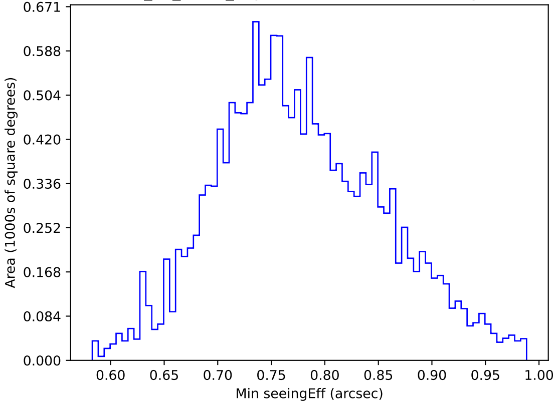
too_10_1v3.4_10yrs WFD u band: Min seeingEff
