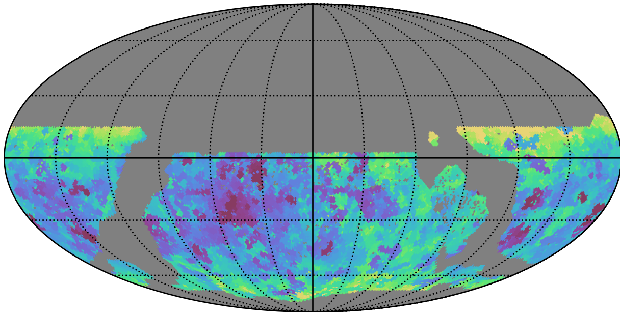
too_10_1v3.4_10yrs WFD r band: Min seeingEff
