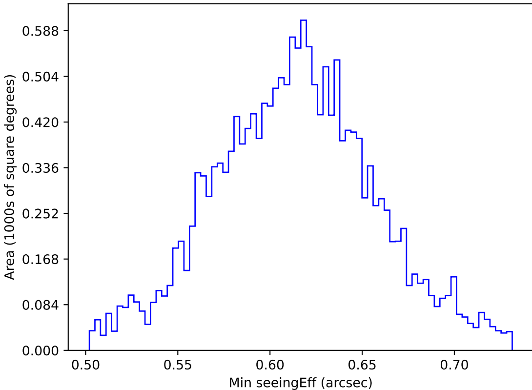
too_10_1v3.4_10yrs WFD r band: Min seeingEff
