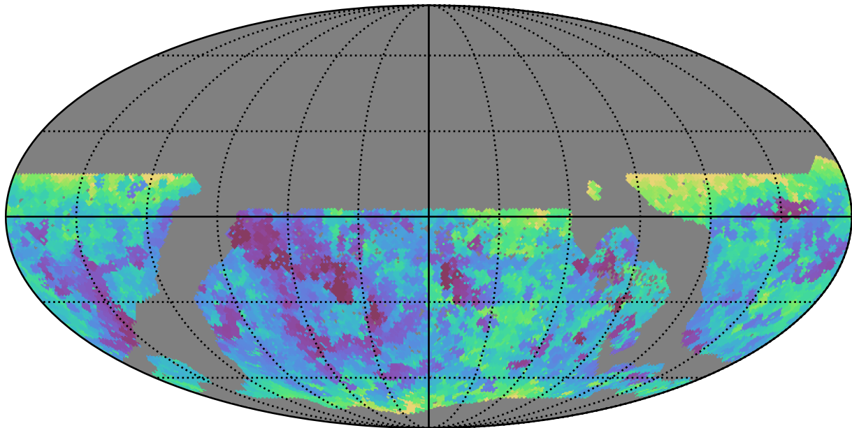
too_10_1v3.4_10yrs WFD i band: Min seeingEff
