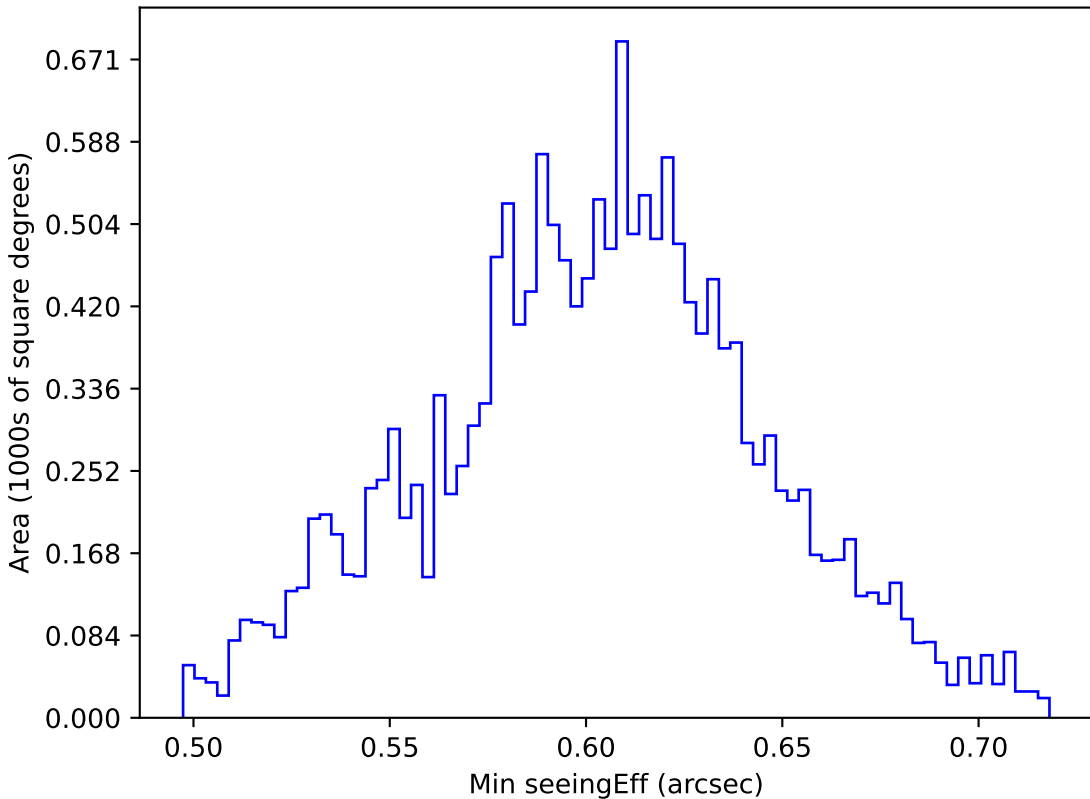
too_10_1v3.4_10yrs WFD i band: Min seeingEff
