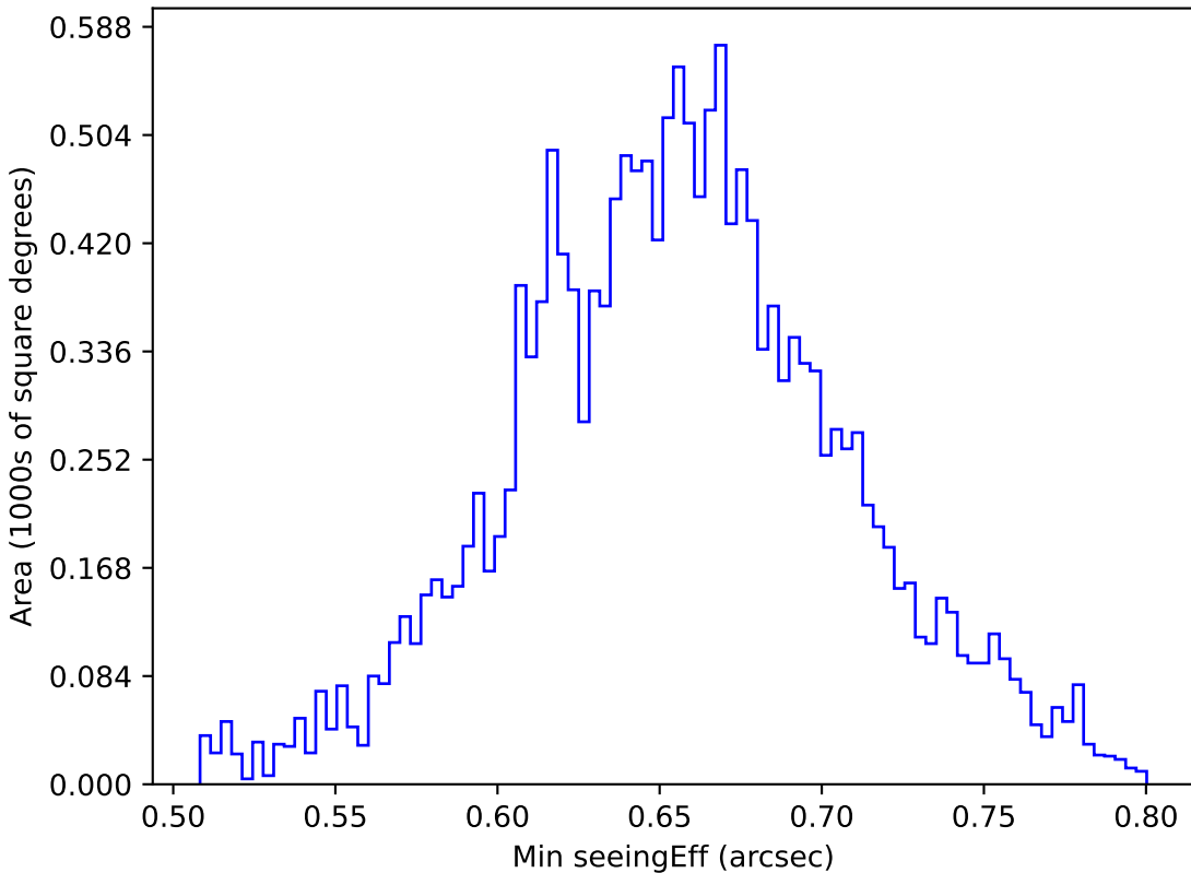
too_10_1v3.4_10yrs WFD g band: Min seeingEff
