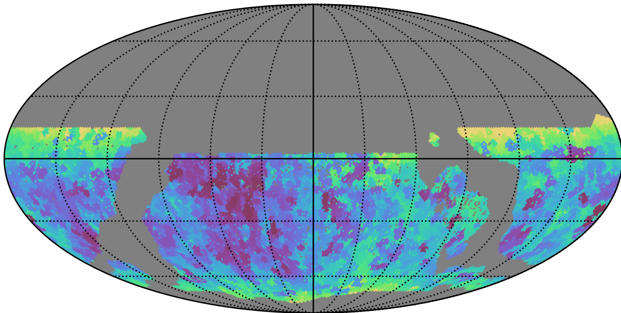
too_10_1v3.4_10yrs WFD all bands: Min seeingEff
