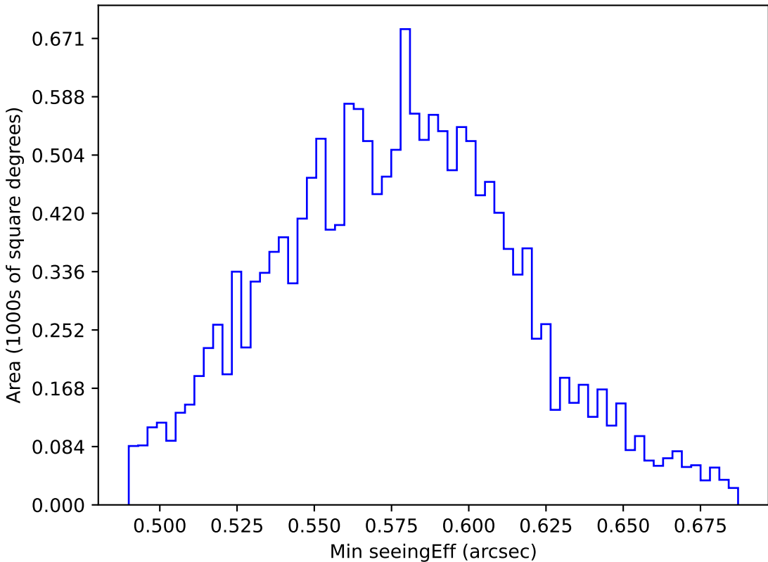
too_10_1v3.4_10yrs WFD all bands: Min seeingEff
