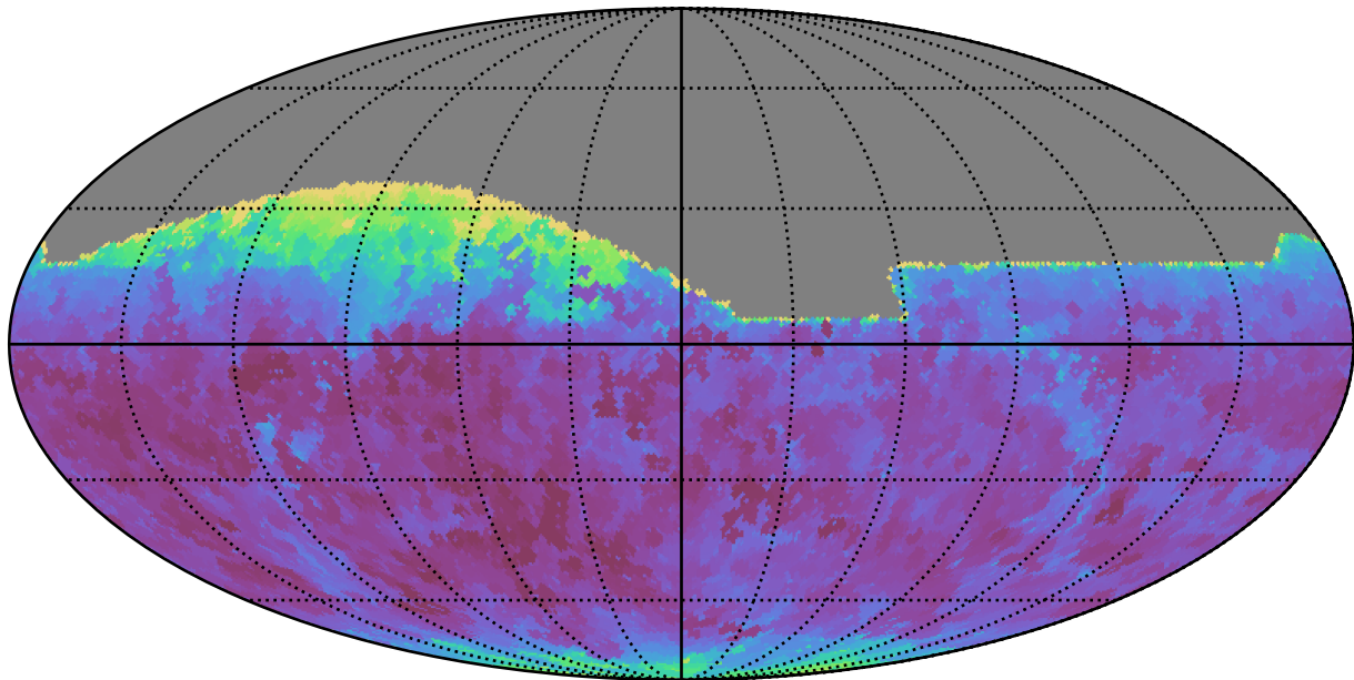
too_10_1v3.4_10yrs All sky z band: Min seeingEff
