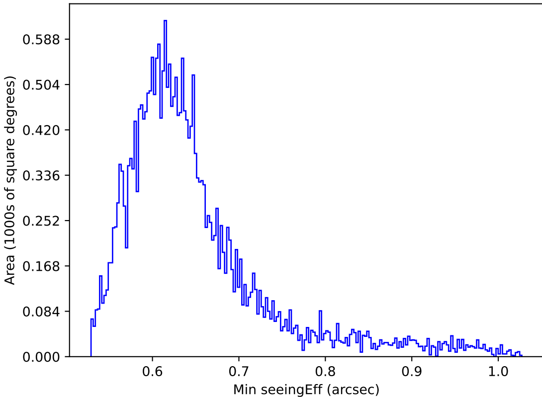
too_10_1v3.4_10yrs All sky z band: Min seeingEff
