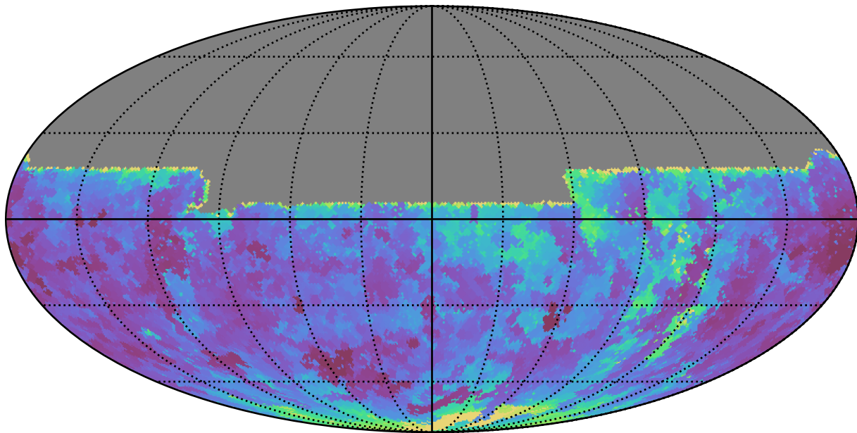
too_10_1v3.4_10yrs All sky u band: Min seeingEff
