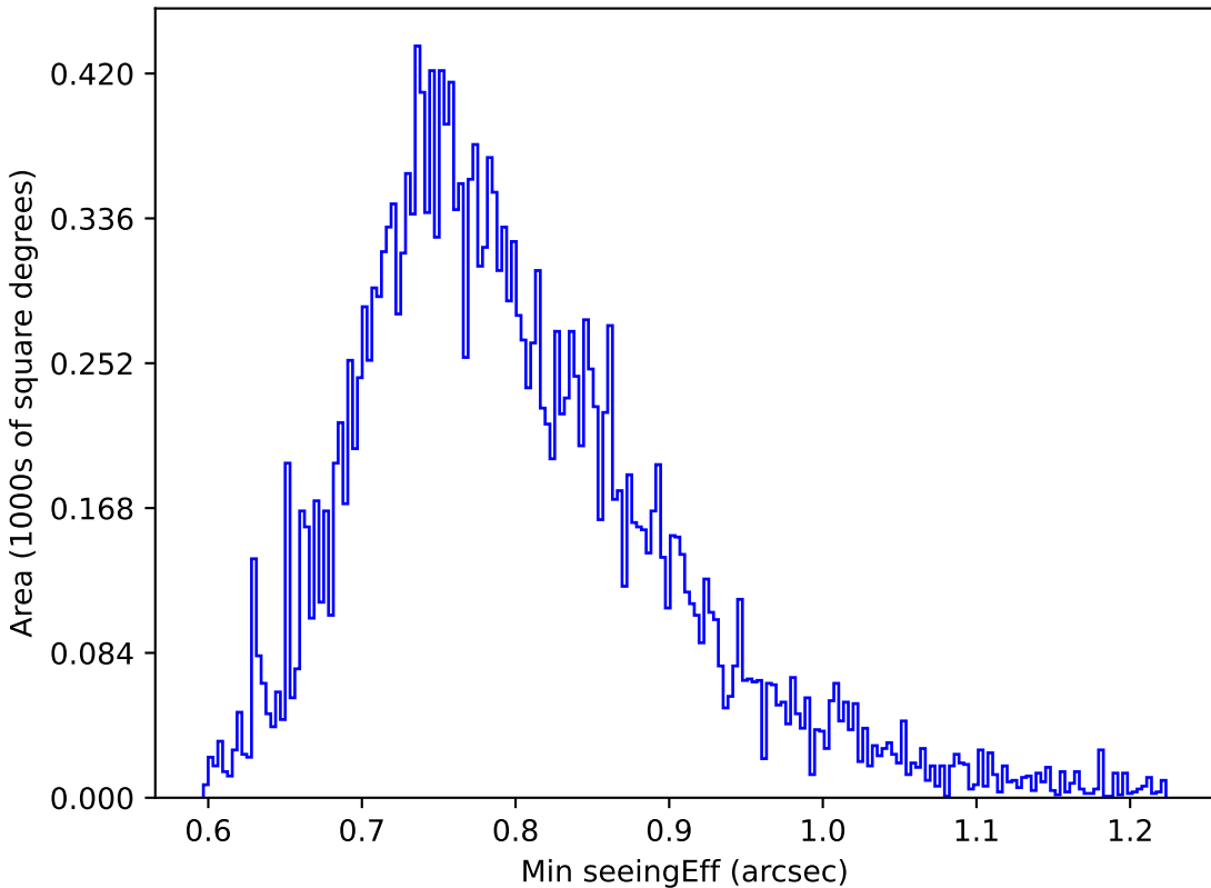
too_10_1v3.4_10yrs All sky u band: Min seeingEff
