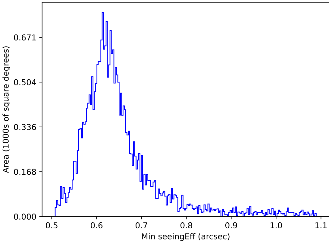
too_10_1v3.4_10yrs All sky r band: Min seeingEff
