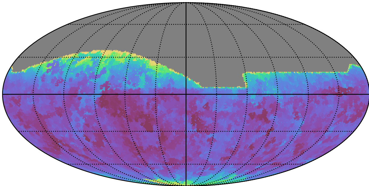
too_10_1v3.4_10yrs All sky i band: Min seeingEff
