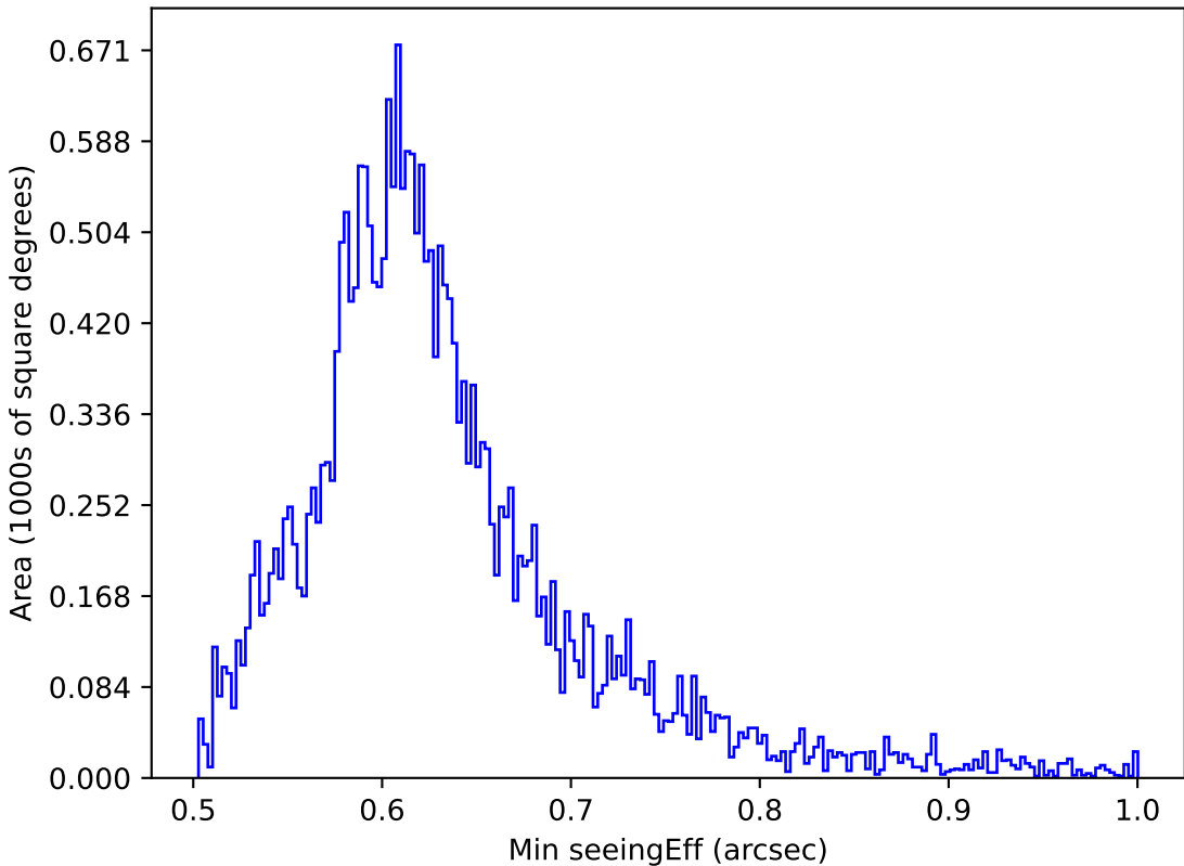
too_10_1v3.4_10yrs All sky i band: Min seeingEff
