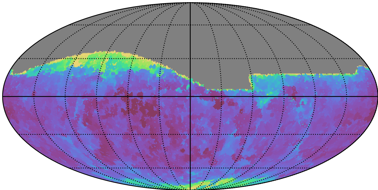
too_10_1v3.4_10yrs All sky g band: Min seeingEff
