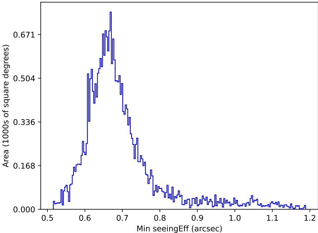
too_10_1v3.4_10yrs All sky g band: Min seeingEff
